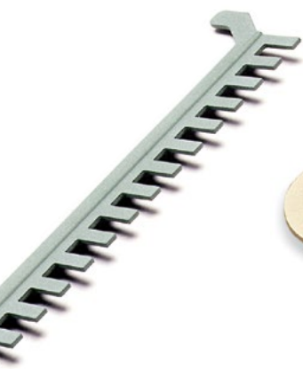
.020" Thick Stainless Steel. Indexed Plate. Photoetched Blank. Die Formed and Teflon Coated.
