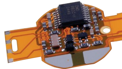
SMT Assembly
