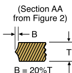
Figure 1 Typical Etched Edge
